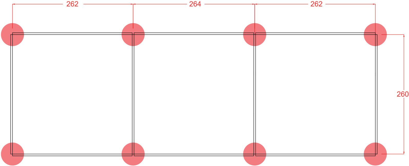
Top view
