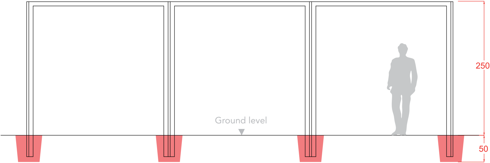
Front view
